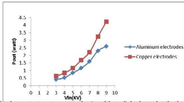
Fig. 3: The plasma actuator out power as a function of the applied voltage when the electrodes material is Copper and Aluminum, and the dielectric material is PMMA.
