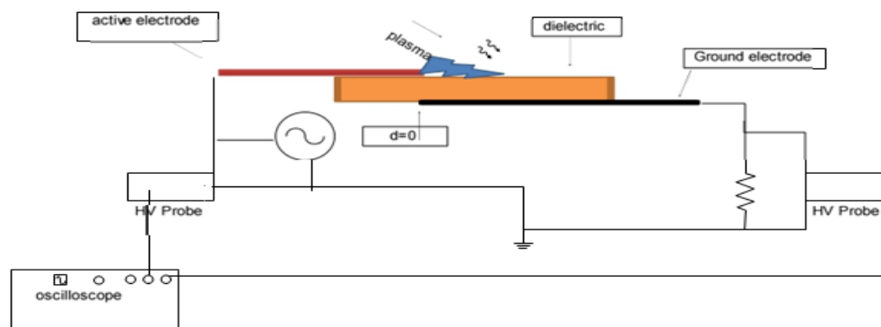
Fig. 1: Single dielectric barrier discharge plasma actuator setup.
